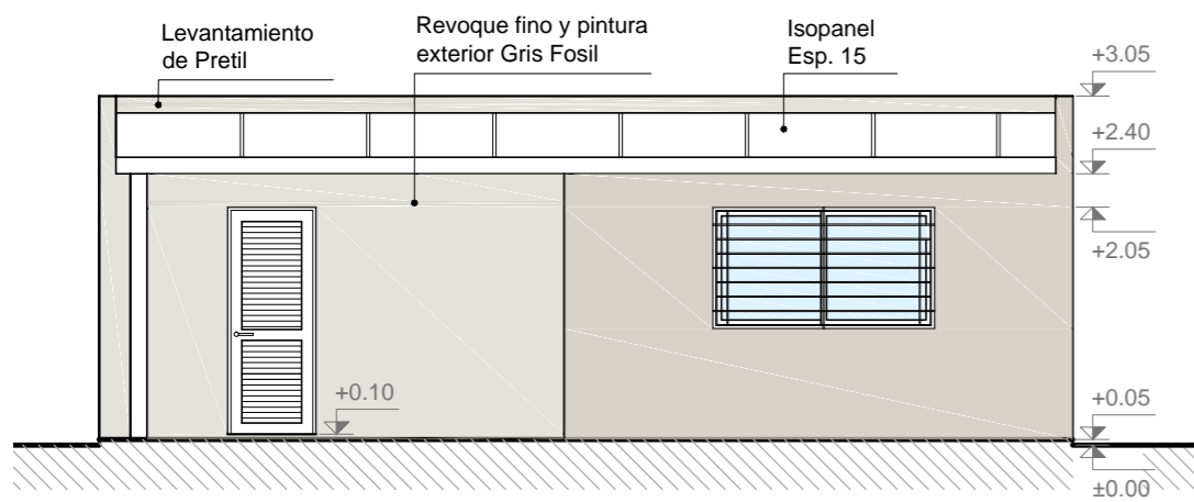
FACHADA PRINCIPAL
