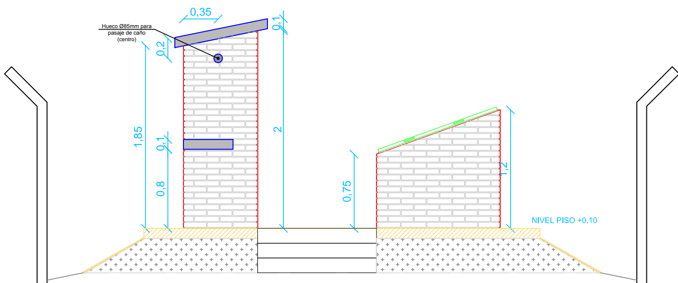
FACHADA PRINCIPAL
