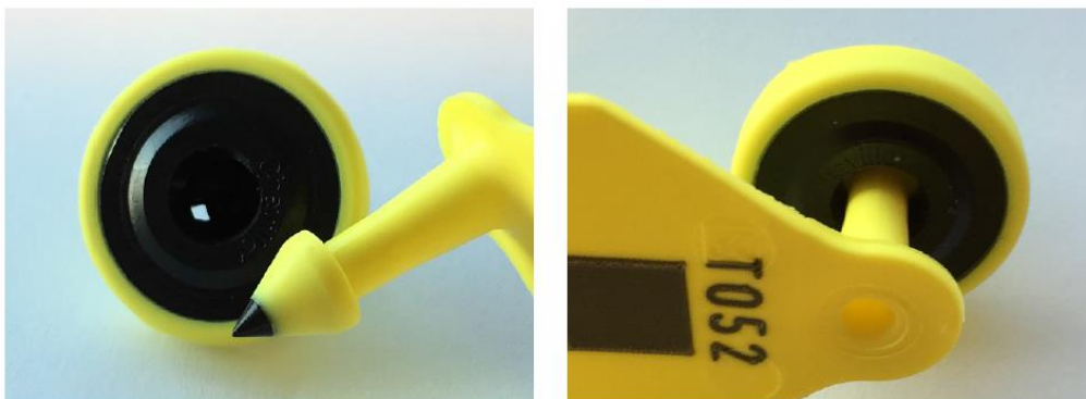
Figure 2a/b: locking mechanism of T052 ear tag
